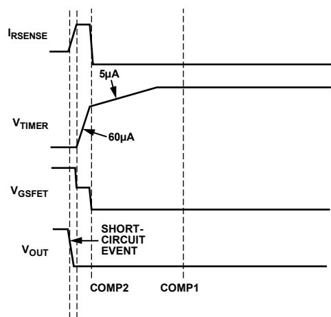
Figure 33. ADM4210-2 Latch Off After Overcurrent Fault
