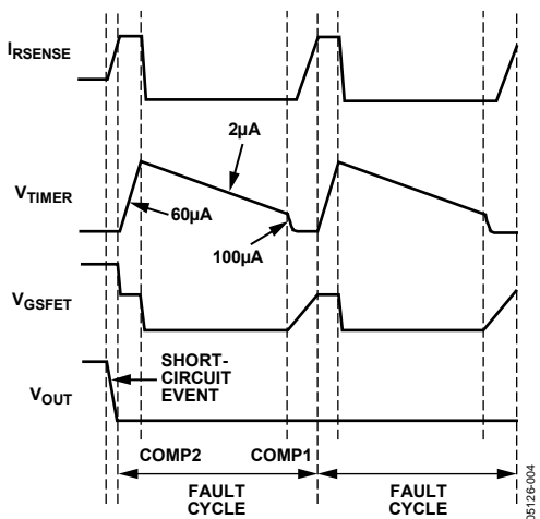
Figure 32. ADM4210-1 Automatic Retry During Overcurrent Fault
