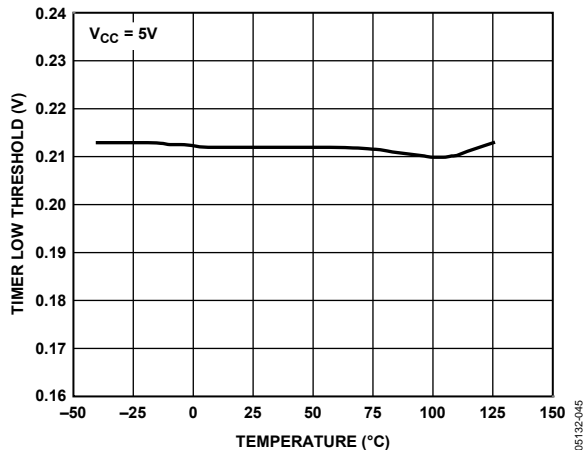
Figure 23. TIMER Low Threshold vs. Temperature
